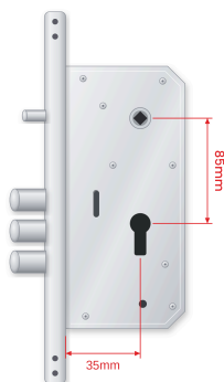
3585 lock body
