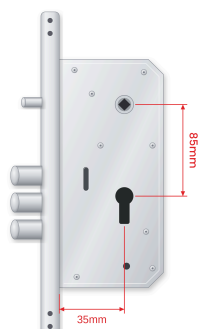
3585 lock body
